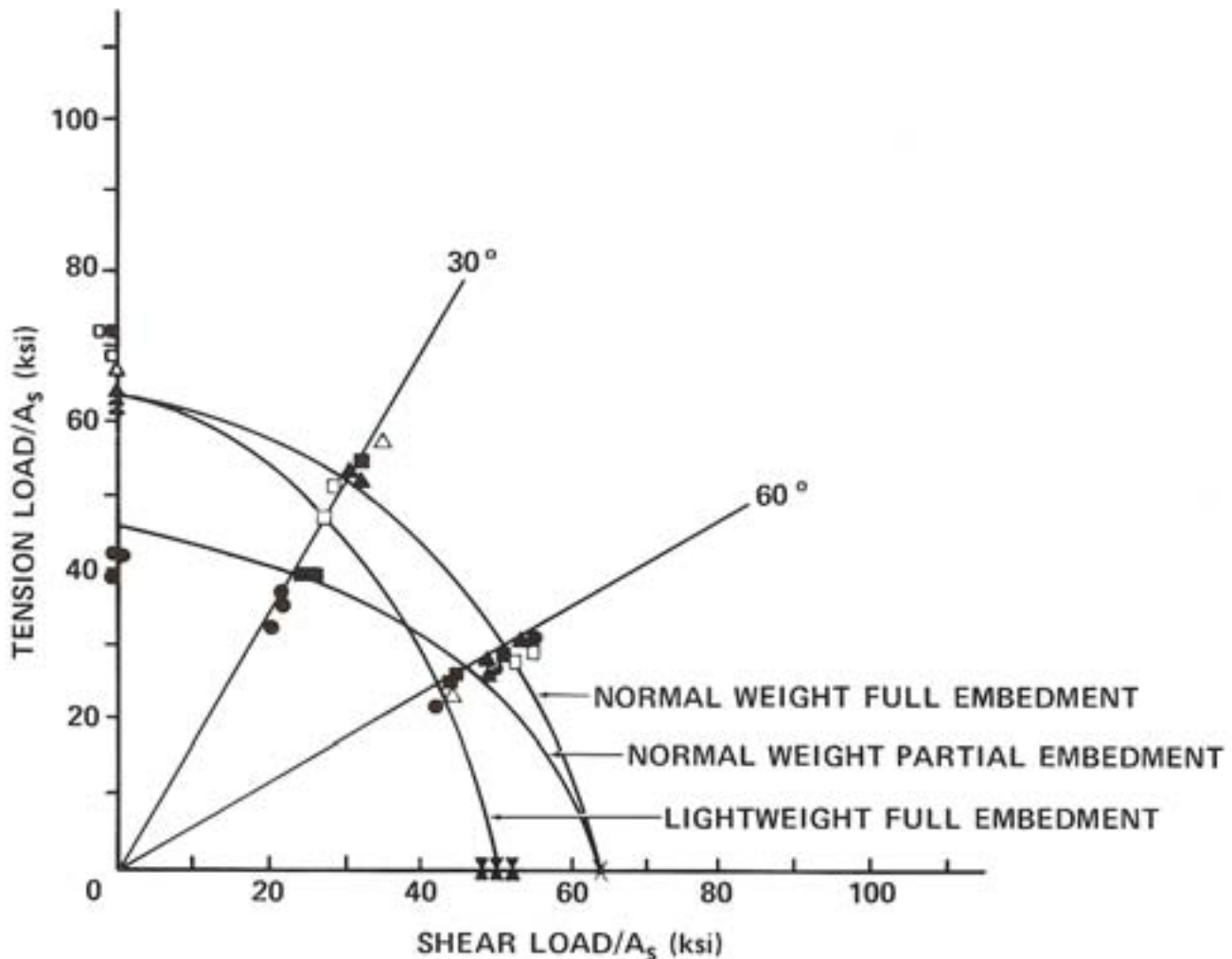
FIGURE 29.— Combined Loading — Formulae Versus Test Data.
