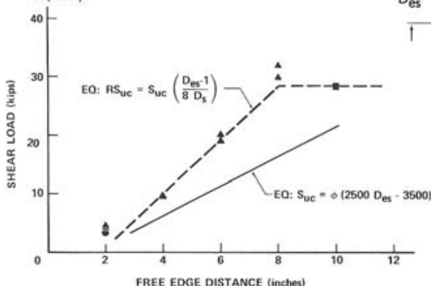
FIGURE 20.—Reduced Shear Capacity — Free Edge Condition Subject to Shear Force
