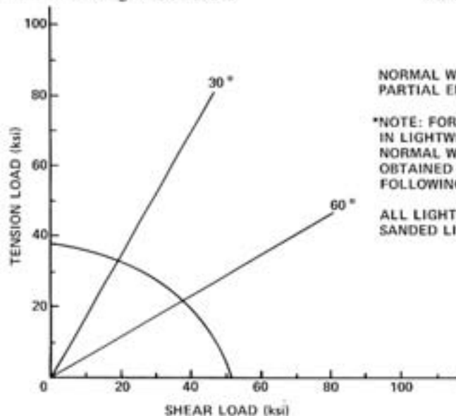
FIGURE 30.—Interaction Design Curve. Combined Loading of Full Embedment Anchors in Normal Weight Concrete
