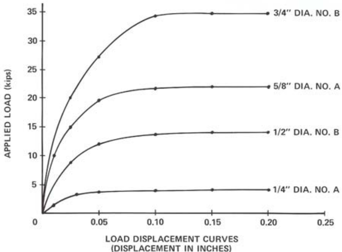
FIGURE 1. — Load Displacement Curves
