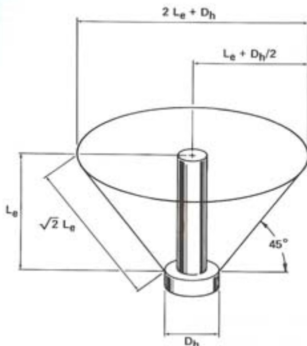
FIGURE 4.—Partial Embedment — Full 45° Shear Cone
