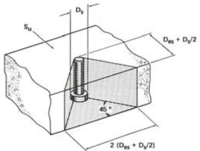
FIGURE 22.—Geometry of Free Edge Shear Failure.
