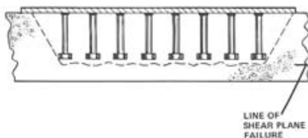
FIGURE 15. — Shear Plane Failure
