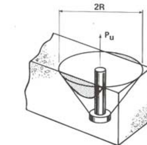
FIGURE 10. — Two Reductions to Full Shear Cone
