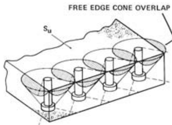
FIGURE 25.—Reduced Shear Capacity at Free Edge Due to Cone Overlap.
