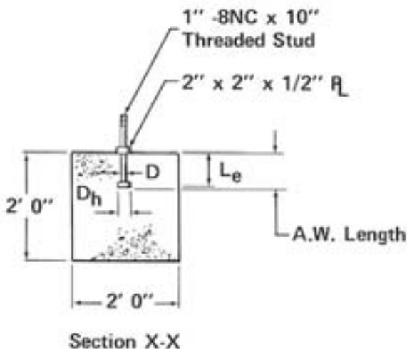
FIGURE 6.—Typical Test Beam and Anchor Test Schedule
