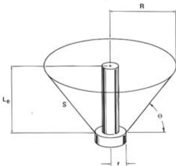
FIGURE 3. — Full Concrete Shear Cone
