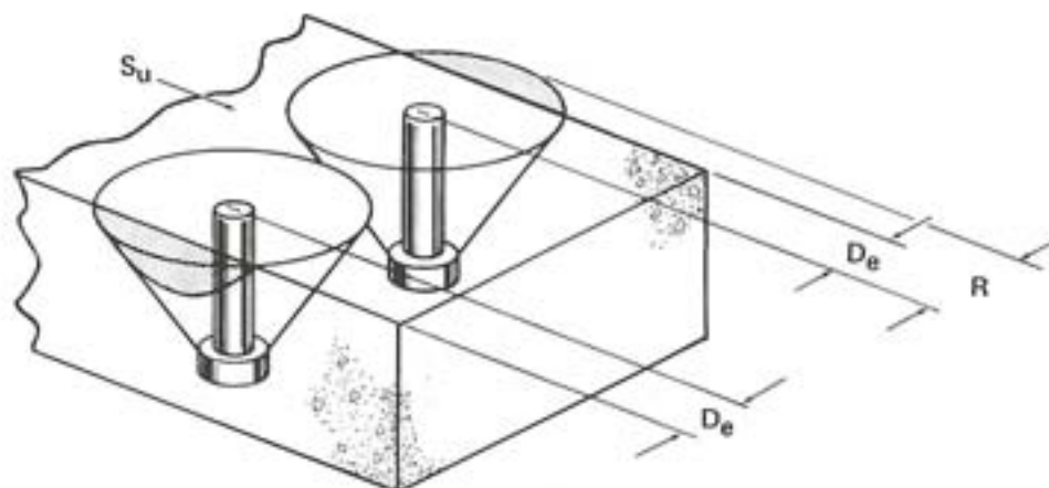
FIGURE 17.—One Reduction To Shear Capacity.
