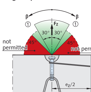
Load capacity and reinforcement for the spherical head eye anchor
